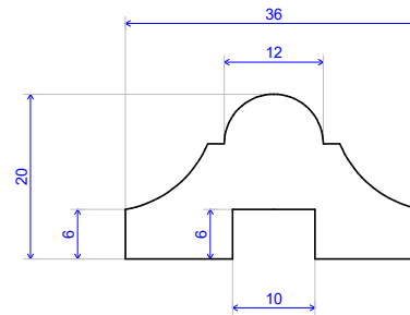
Profile No. 130236
