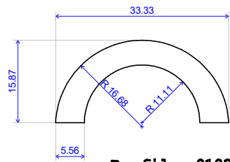
Profile: 01038
