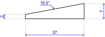
Profile No. 130952
