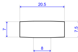
Profile No.131247
