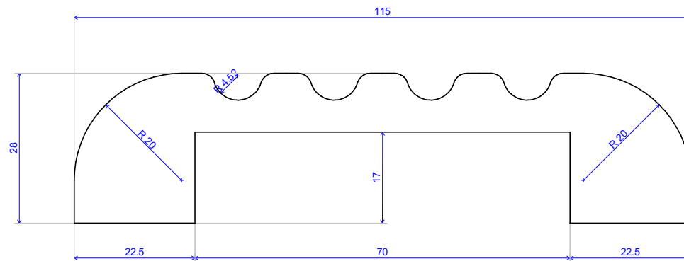
Profile No .132140
